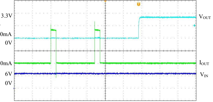
Short Circuit Protection ( V_{IN}=6V V_{OUT}=\text{short to } 3.3V )
